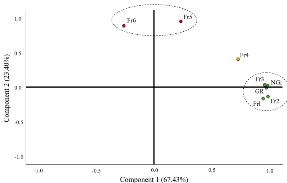
Fig. 8. Loading plot of principal components PC1 and PC2 for the Azorean Cryptomeria japonica immature female cones essential oil (EO) and EO fractions (Frs. 1–6). GR and NGr: grinded and non-grinded plant material, respectively.
