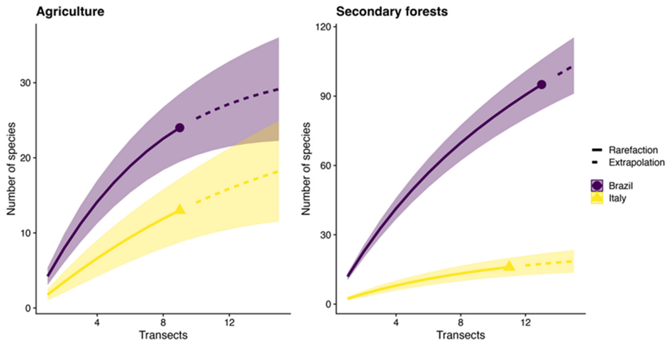
Figure 1. Species rarefaction curves for ants sampled in agricultural and secondary forests in Brazil and Italy. The solid and stippled lines represent the interpolated and extrapolated values, respectively. Shaded areas around the lines represent the 95% confidence intervals.
