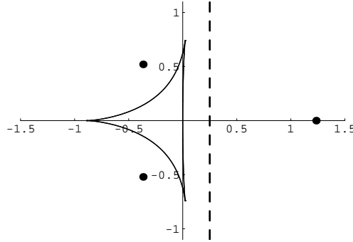
Figure 4. Curve of C2 type with a deltoid and a double tangent (at complex points) of equation x = 1/4 .
