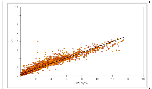
Figure 2. Observed UVI values vs. modeled ( G \cdot UVI_0 / G_0 ) for cloudy sun cases (Global/Diffuse <1.1)
