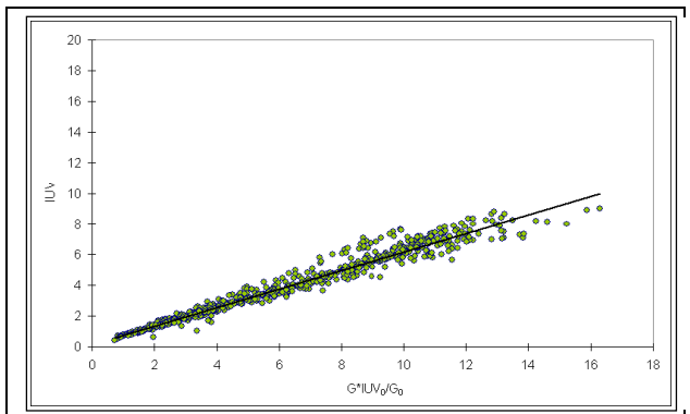
Figure 1. Observed UVI values vs. modeled ( G \cdot UVI_0 / G_0 ) for direct sun cases (Global/Diffuse >5)
