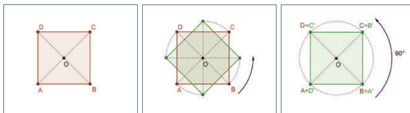
Figure 1: Rotational symmetry.
