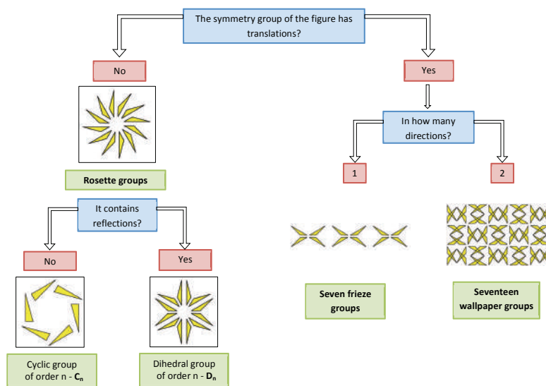
Figure 4: Symmetry groups.
